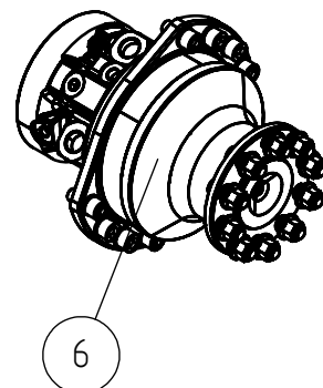
VASEN TAKAMOOTTORI Left rear drivemotor
